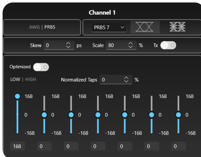
Figure 7: Channel Configuration
