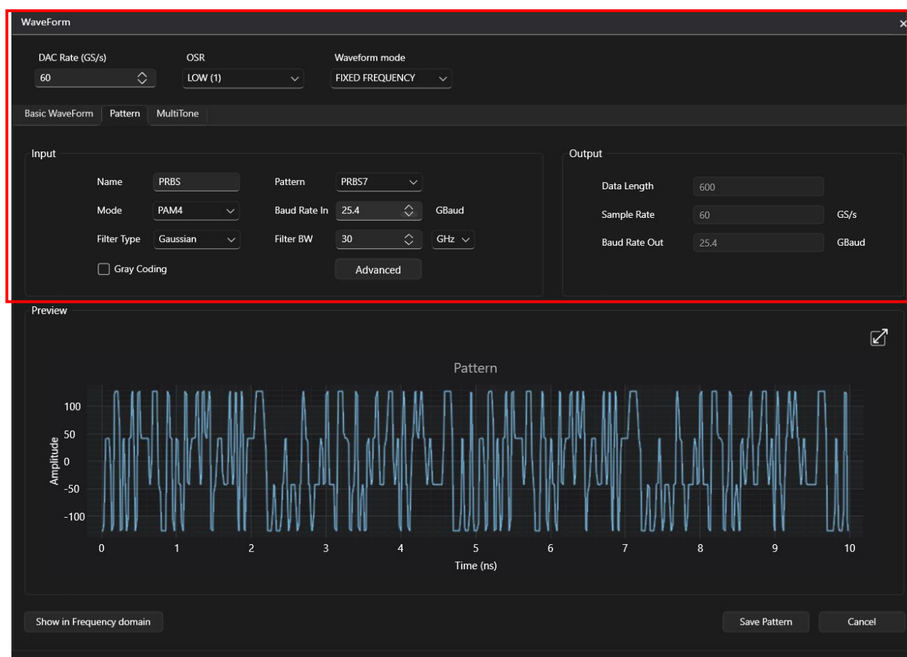
Figure 32:Pattern parameters
